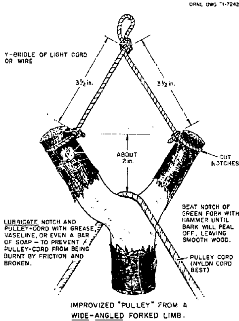
Fig. B-17. Improved pulley from a wide-angled forked limb.
